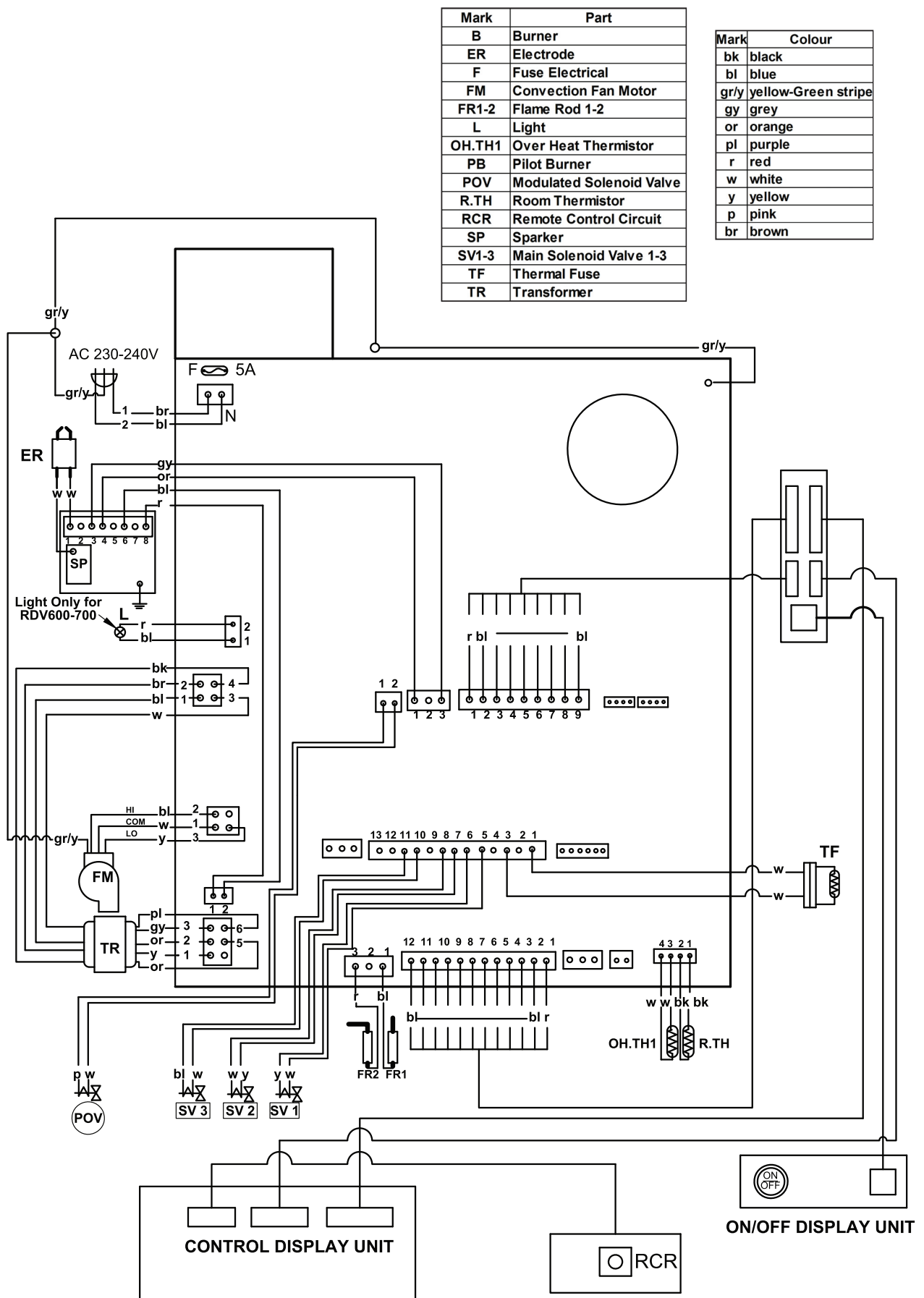
WIRING DIAGRAM UNI CONTROL MODEL 3 1 Burner Issue B
