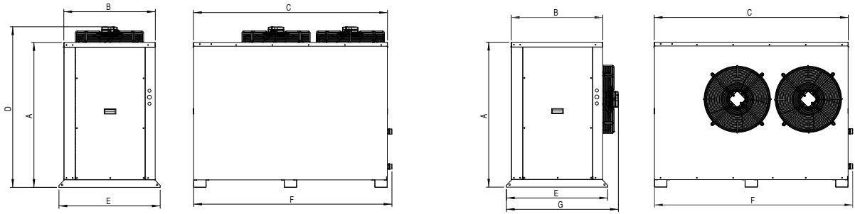
Top Discharge Unit
