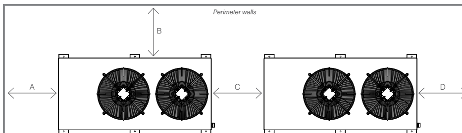
Top Discharge Unit (plan view)
