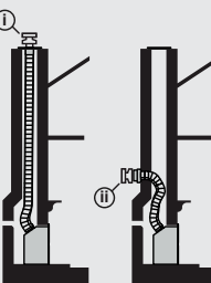
Masonry i. Vertical ii. Horizontal
