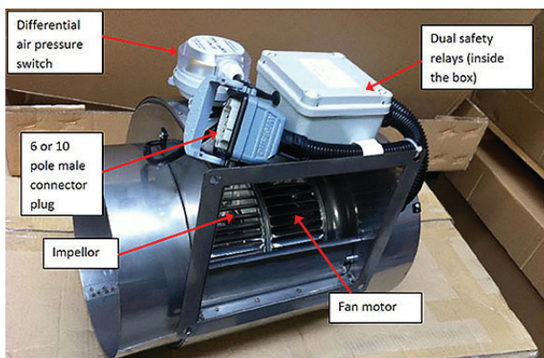
Figure 9. Fan and Air Flow Switch
