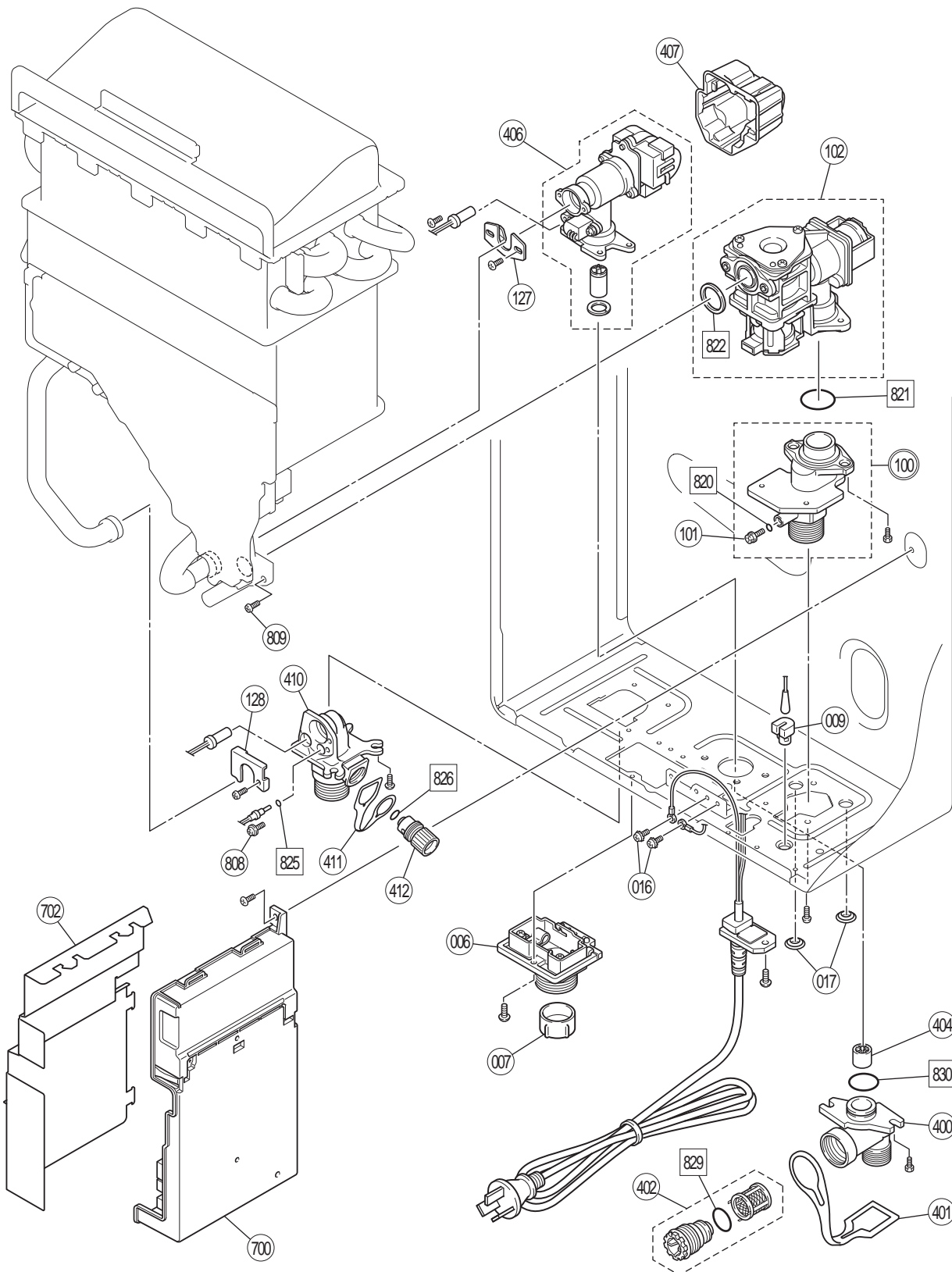
REU-AM2626WD-AK SERIES EXPLODED VIEW-INTERNAL(OUTDOOR) ILLUSTRATION REPRESENTS 2626 MODEL
