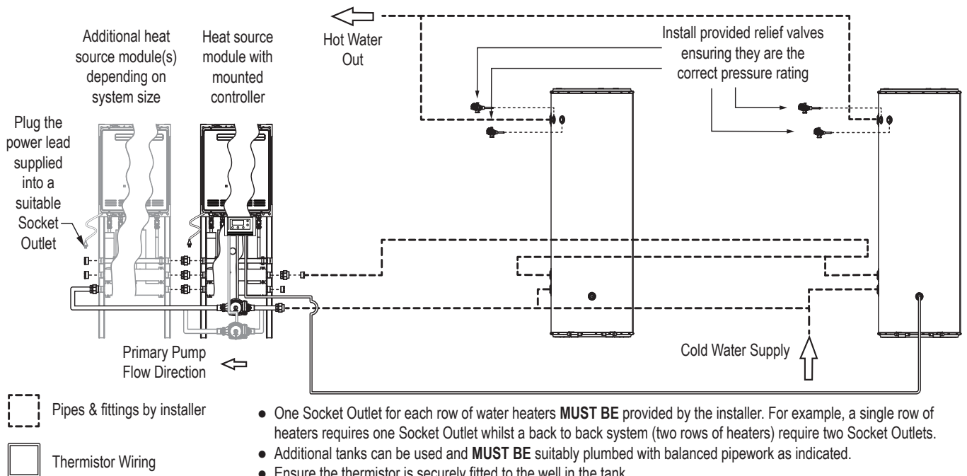
Figure 6. Demand Duo PLUS (Additional Tank)
