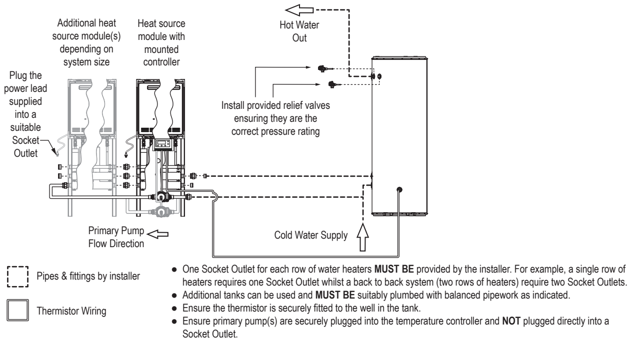
Figure 5. Demand Duo PLUS
