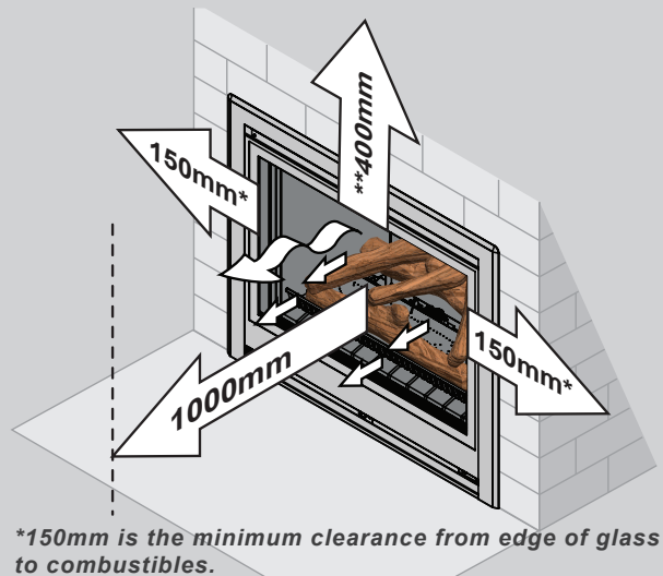
**400mm is the minimum top clearance from edge of glass to combustible items other than mantel, overhanging 250mm or less. (Refer Mantel Clearances, page 7 and TV Installation, page 9)
