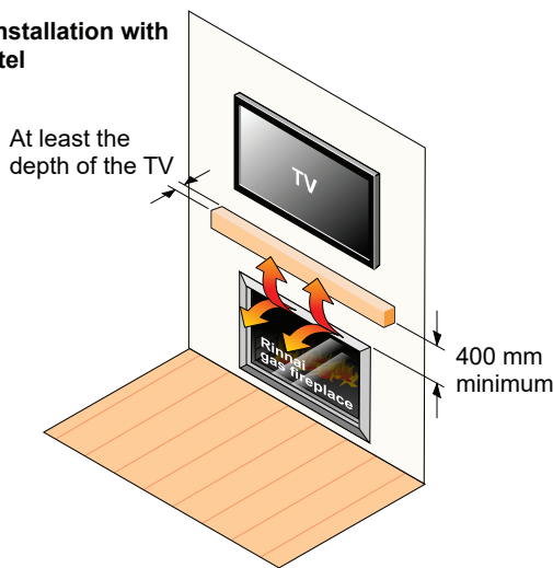
TV Installation with Recess
