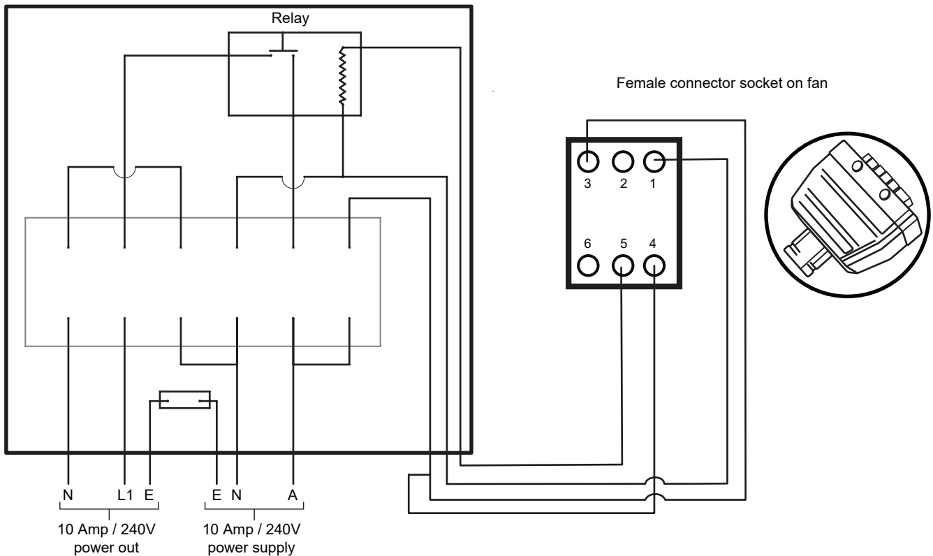
Figure 7. Fan Connection
