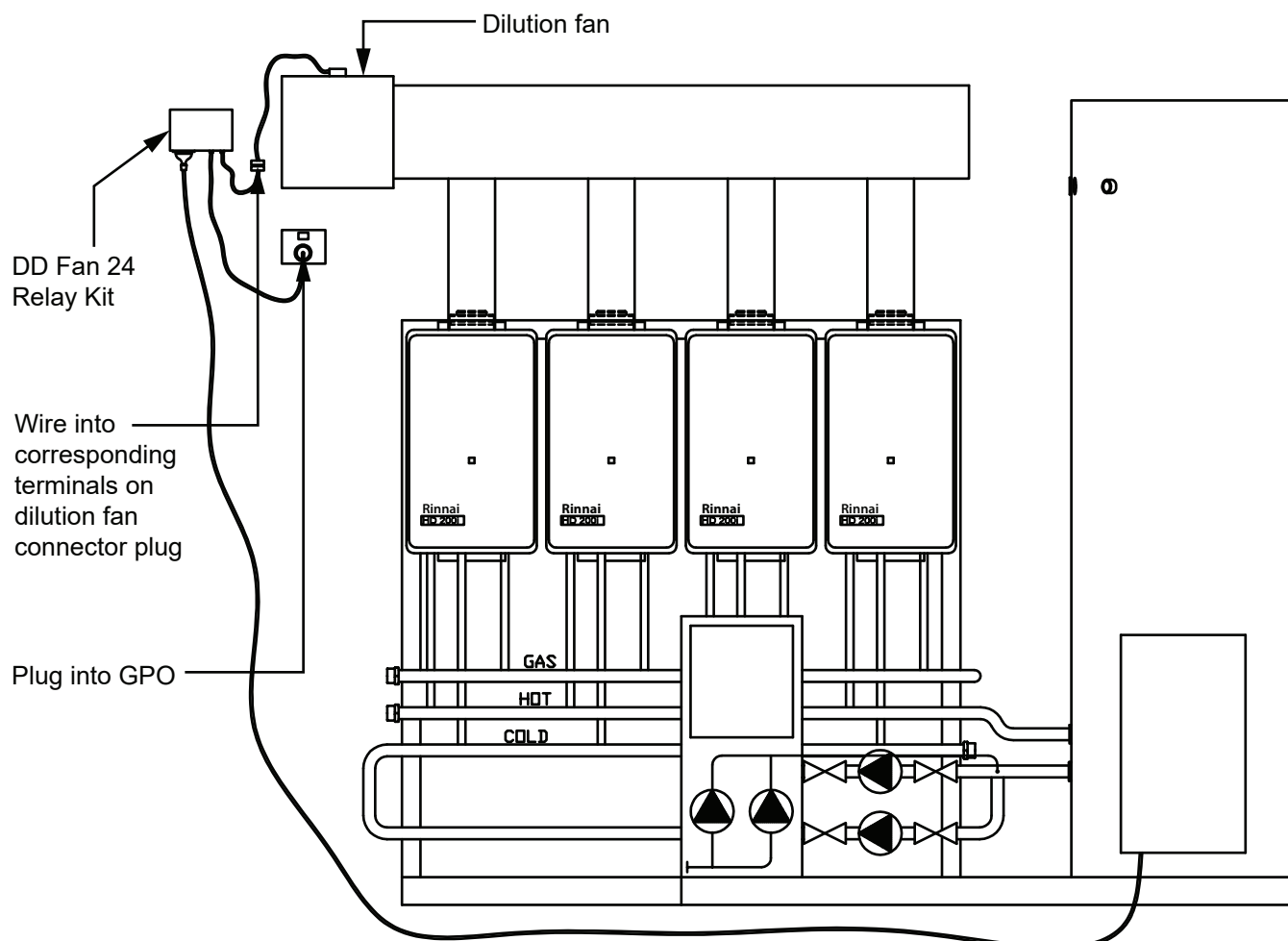
Figure 10. Common Flue Relay Wiring Box
