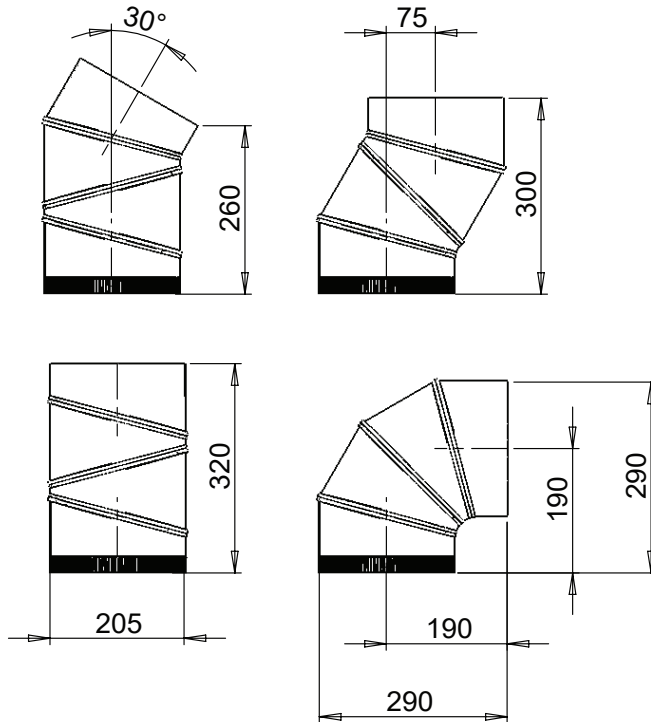
ADJUSTABLE SLEEVE
