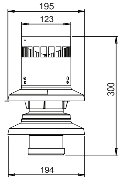
FLUE INSERT TERMINAL
