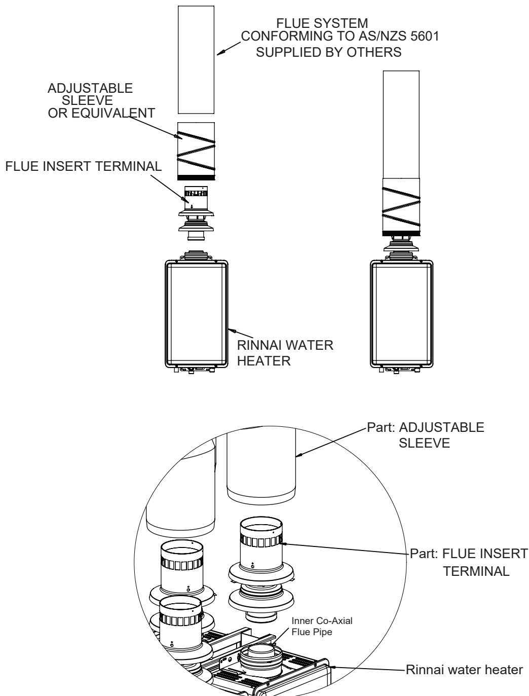
Figure 1. Rinnai Commercial Common Flue System - Components
