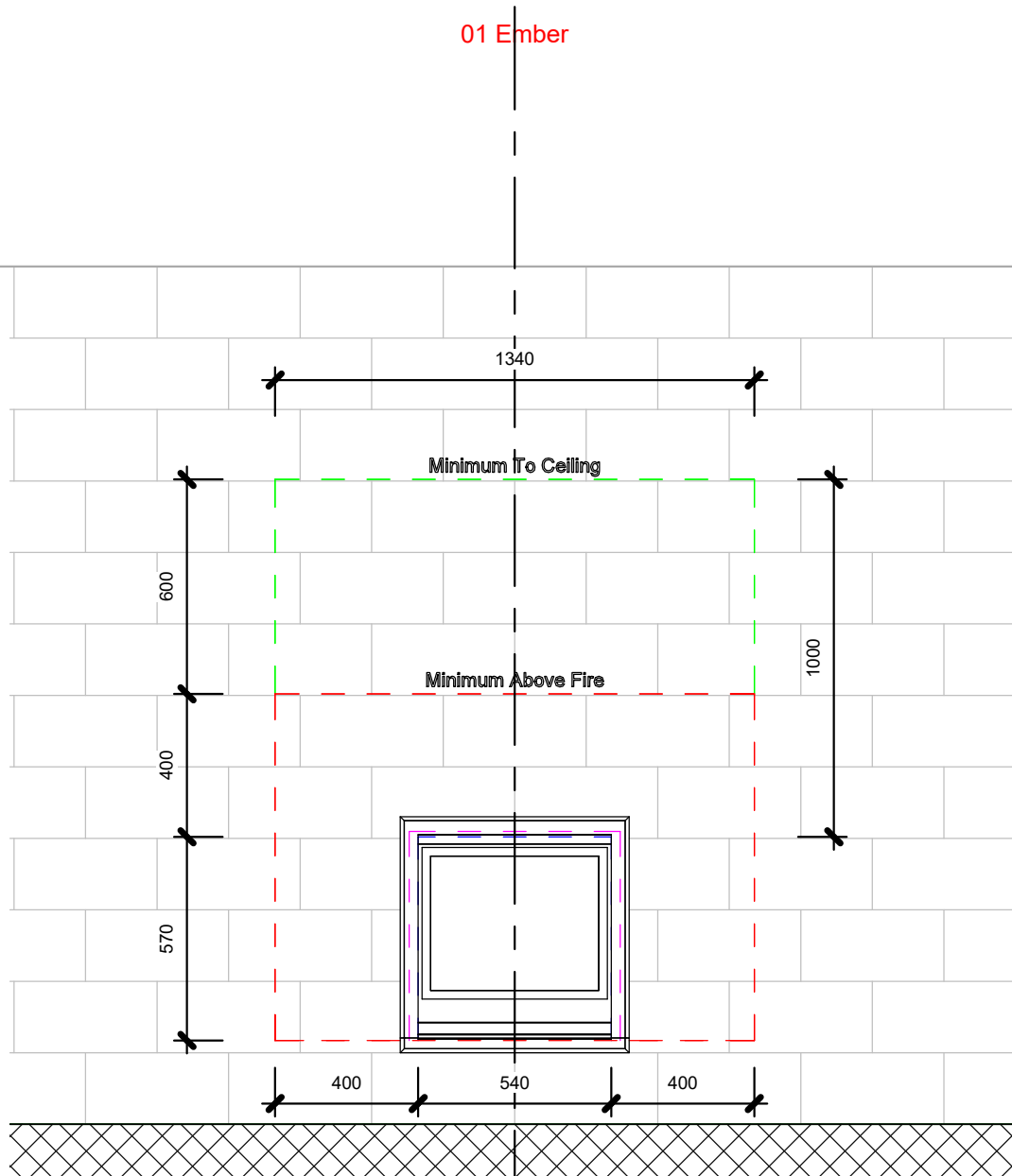
Rinnai Ember 600 Masonry 4 sided front
