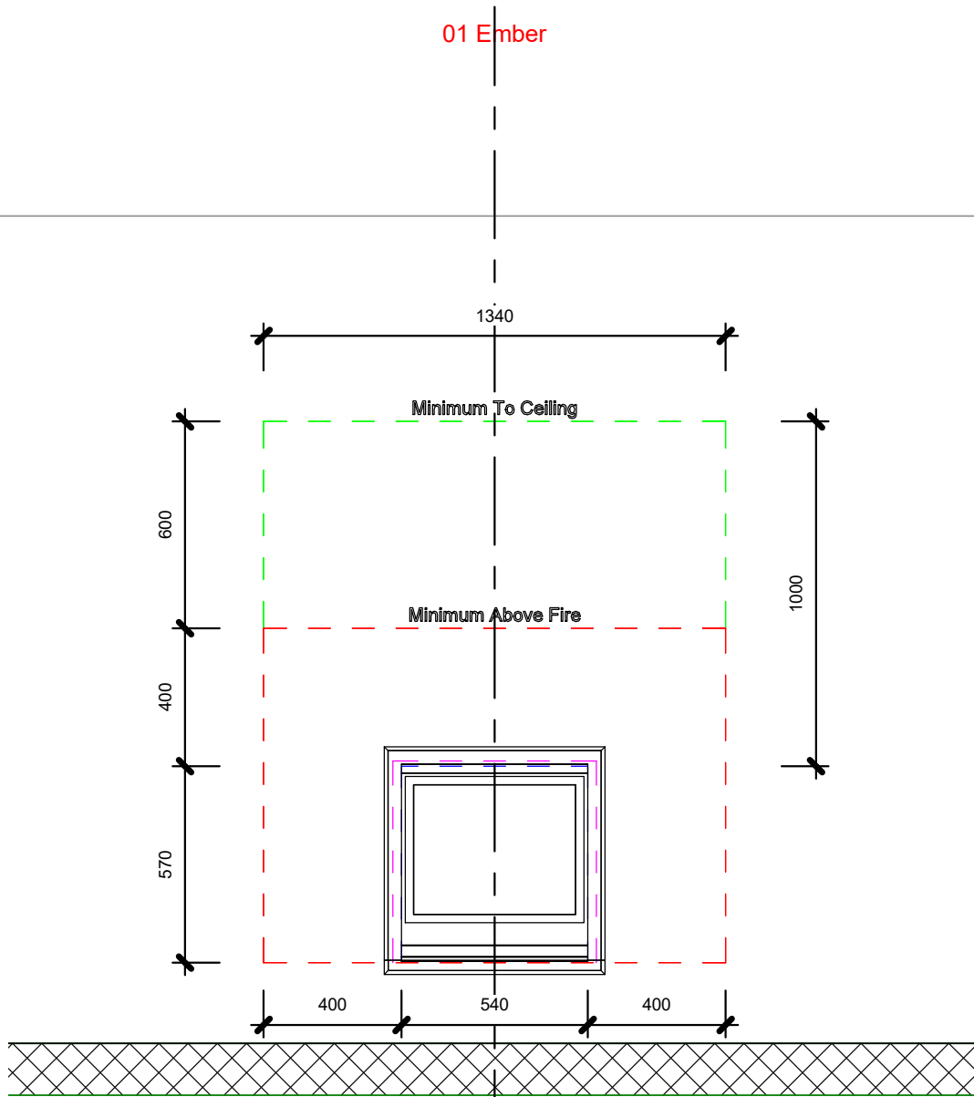
Rinnai Ember 600 Framing 4 sided front
