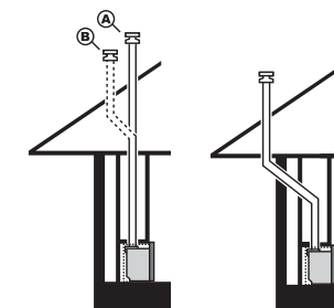
Inbuilt Zero Clearance
