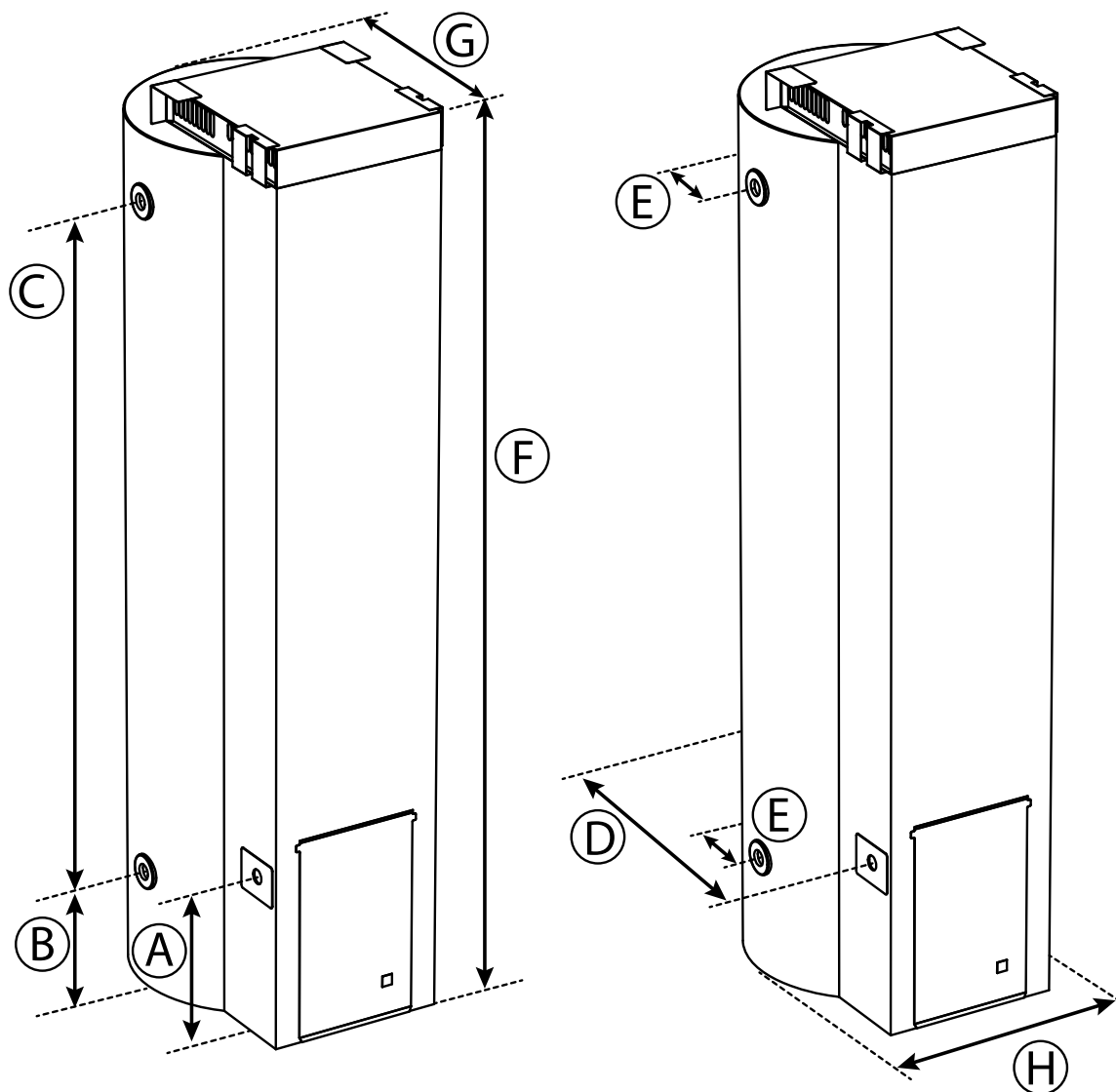
Figure 3 - Appliance Dimensions
