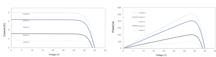
I-V Curve
