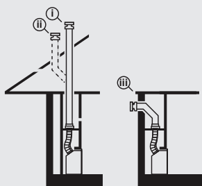
False Fire Place i. Vertical ii. Vertical Offset iii. Horizontal
